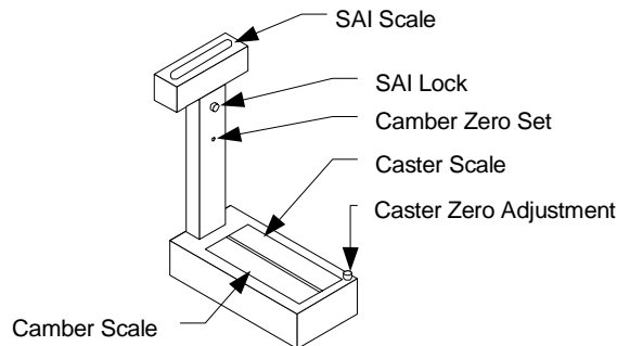
TL-30 Easy Check Gauge
